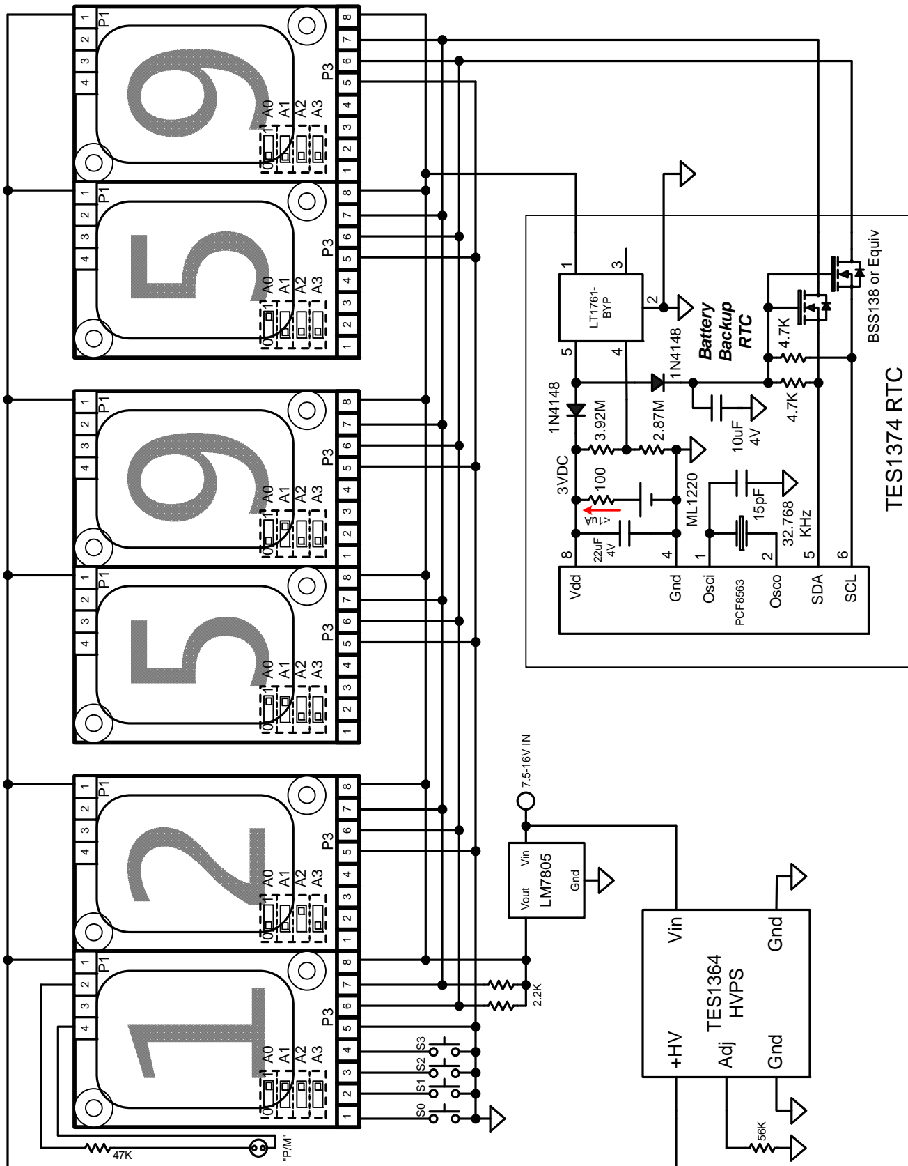
Figure 13: Typical Application, Stand Alone Clock/Calendar (Mode=10)
